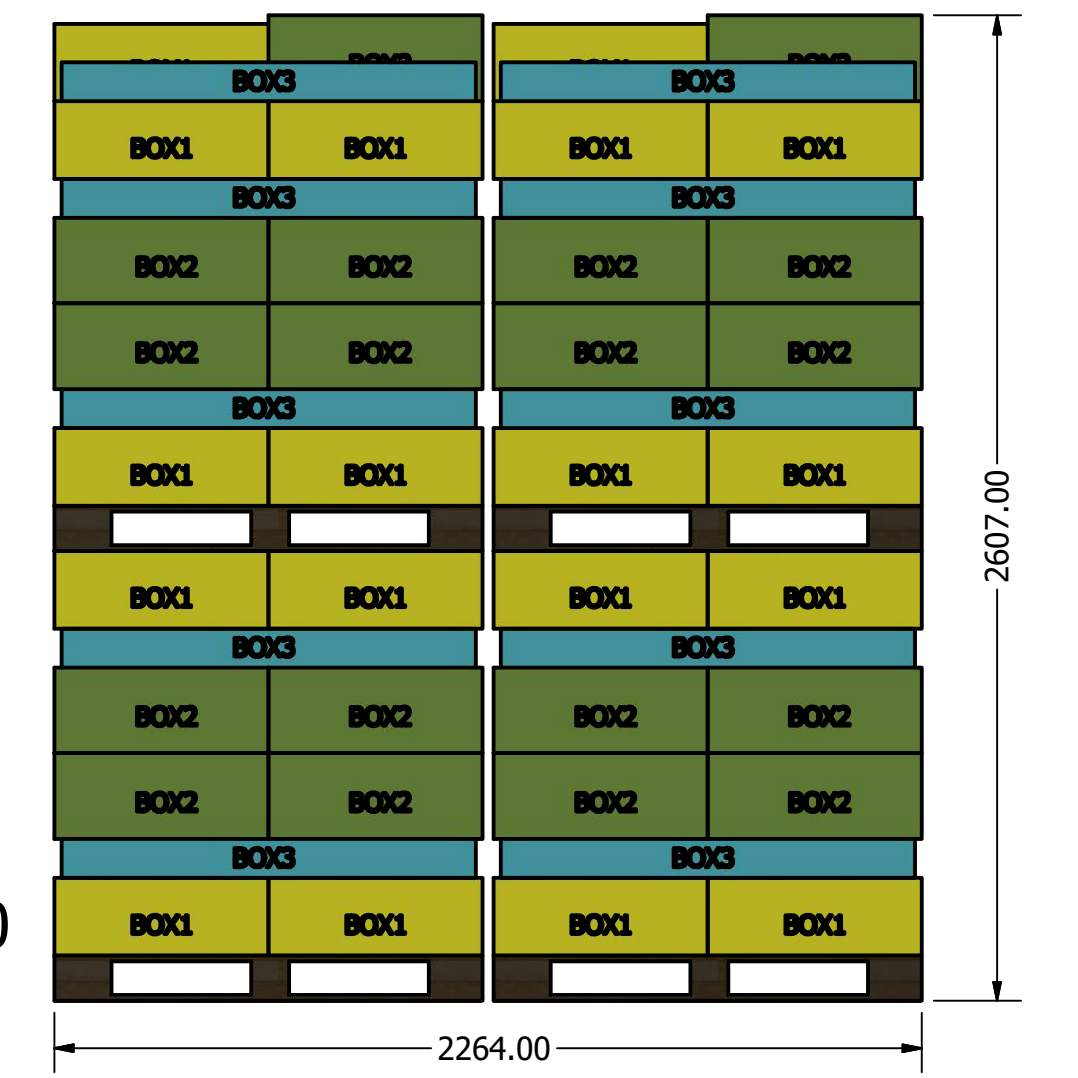
End view
