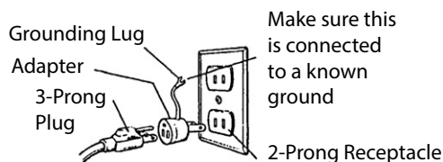
Figure 2 – 2-prong receptacle with adapter.
