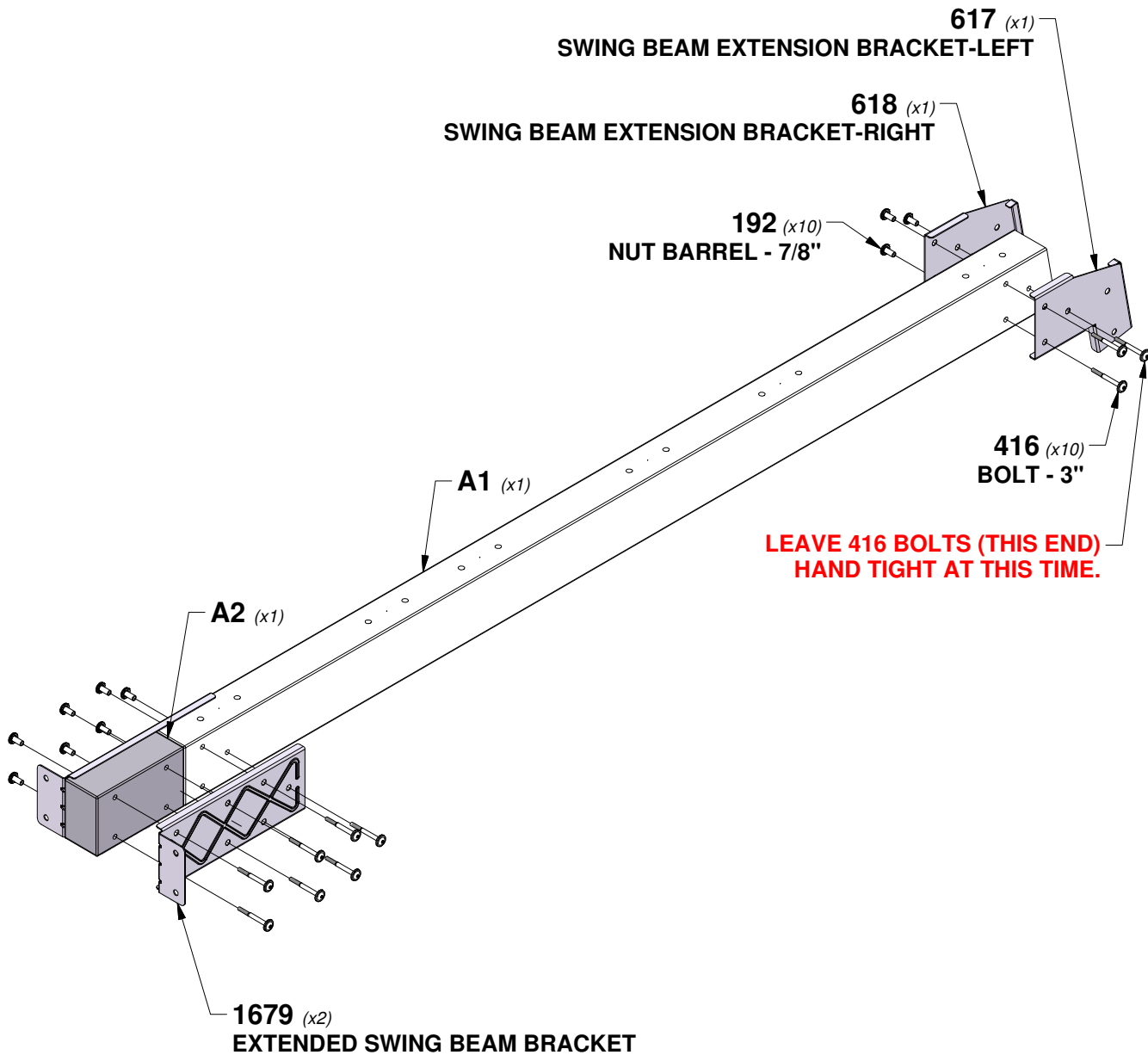
A4M01679 EXTENDED SWING BEAM BRACKET (x2)
