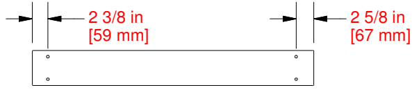
G2 GROUND BOARD - W4L19003 (x1) 1"x5 1/4"x42 1/4" (24x134x1072)
