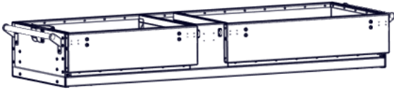
C01 COAL PAN ASSEMBLY - A4M02768 (x1) 11 1/2"x25 9/16"x74 1/2" (292x650x1893)
