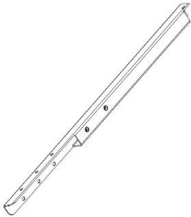
L01 LEG - A4M02912 (x1) 1 1/2"x1 1/2"x31 13/16" (38x38x808)
