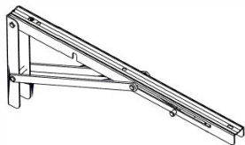
2094 FOLDING TABLE BRACKET - A4M02094 (x4) 1 3/8"x6 13/16"x15 15/16" (34x173x405)
