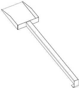
SH01 SHOVEL - A4M02513 (x1) 2 1/4"x4 7/8"x31 7/16" (57x124x798)
