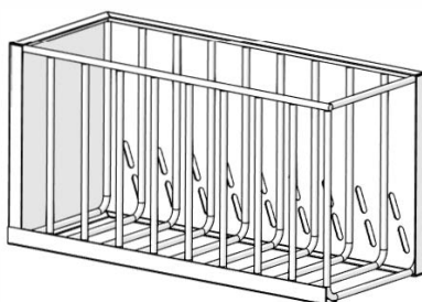
F01 FIRE BOX - A4M02772 (x1) 11 11/16"x9 1/8"x22 1/2" (298x232x572)
