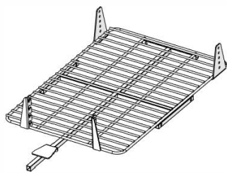
R02 BOTTOM ASADO RACK - A4M02786 (x1) 5 7/16"x18 1/2"x34" (138x470x864)
