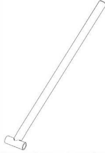
R04 PIVOT ROD - A4M02784 (x1) 1/2"x1 7/16"x12 1/4" (12.0x36x312)
