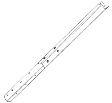
L03 LEG - A4M02914 (x1) 1 1/2"x1 1/2"x31 13/16" (38x38x808)
