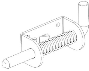
DL01 DOOR LATCH - A4M02496 (x1) 1 5/16"x1 7/8"x4 3/8" (33x47x111)
