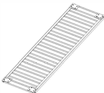
B02 BOTTOM RACK ASSEMBLY - A4M02767 (x1) 1 5/8"x24 1/16"x74 3/4" (40.5x611.5x1898)
