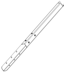
L02 LEG - A4M02913 (x1) 1 1/2"x1 1/2"x31 13/16" (38x38x808)
