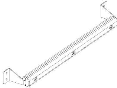
H04 DOOR HANDLE ASSEMBLY - A4M02777 (x1) 2 3/8"x3 3/4"x22 11/16" (60x95x576)
