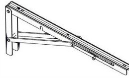
2094 TABLE BRACKET - A4M02094 (x4) 1 3/8"x6 13/16"x15 15/16" (34x173x405)
