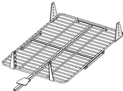
R02 BOTTOM ASADO RACK - A4M02786 (x1) 4 1/4"x18 1/2"x34" (108x470x864)
