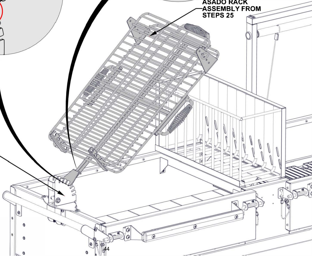
ASADO PIVOT STEPS 25
