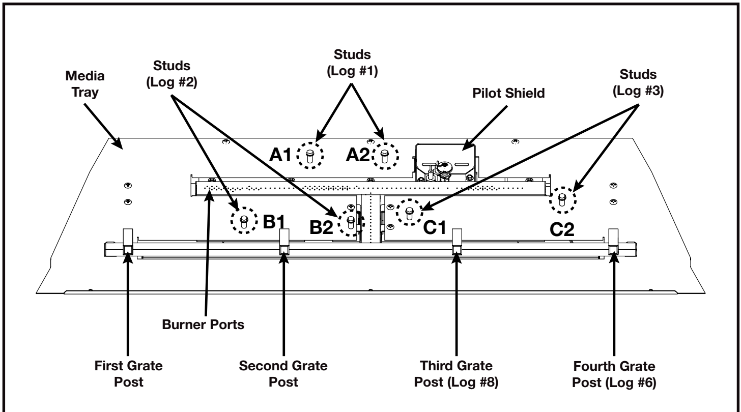
Burner Overview
