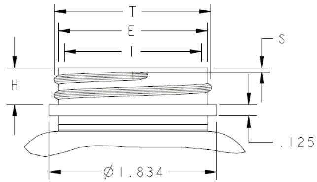
DETAIL A SCALE 3/2
