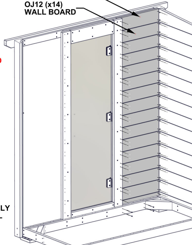
DOOR WALL PANEL ASSEMBLY
