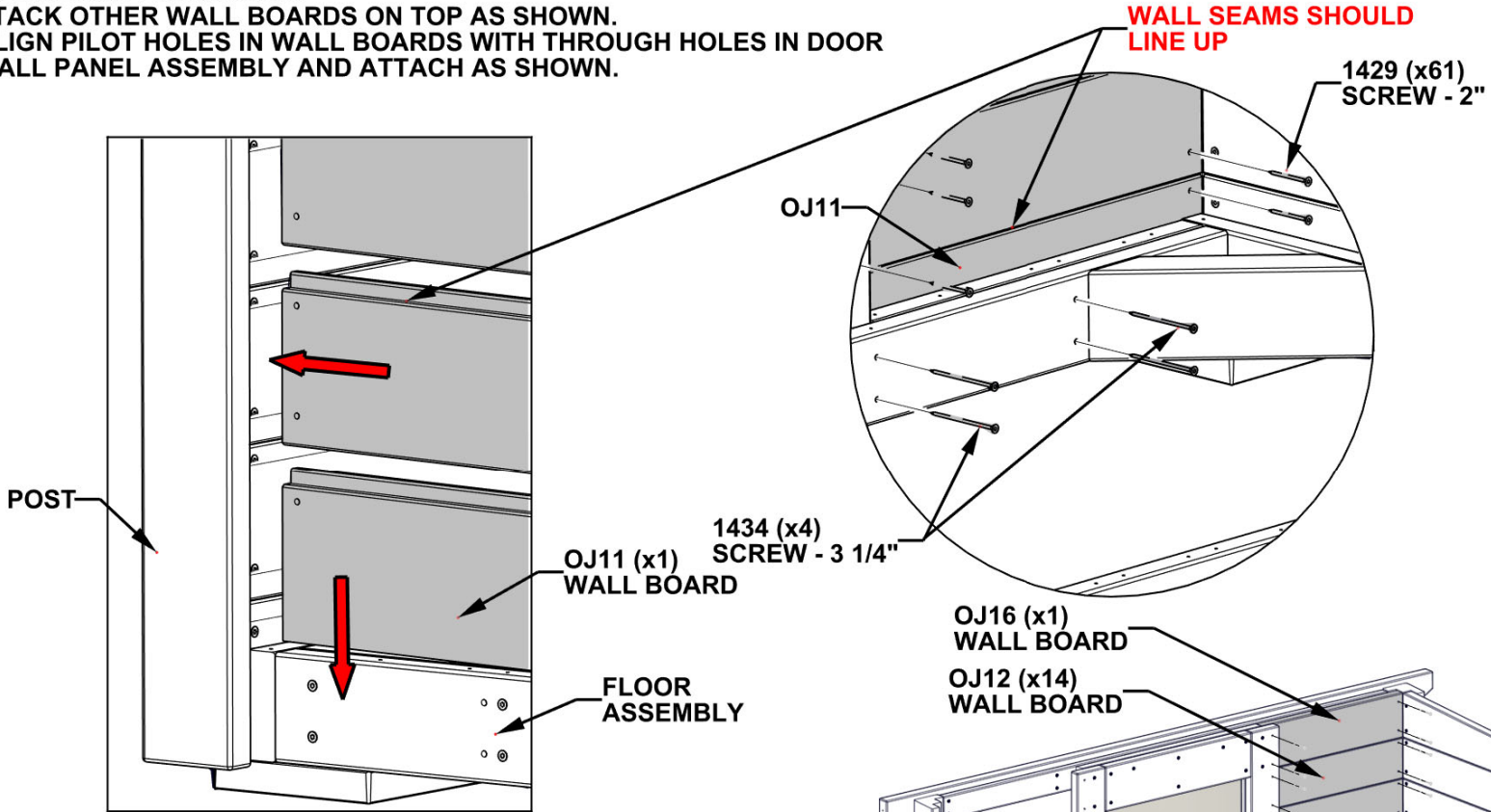
OUTSIDE VIEW
