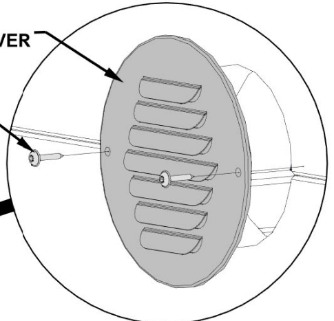
1438 (x4) SCREW - 3/4"
