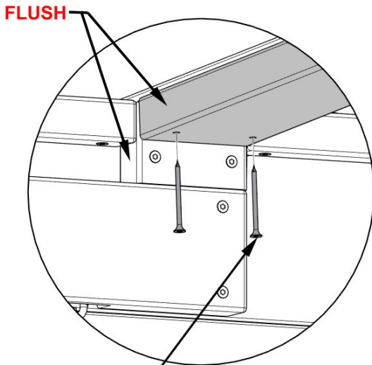
1429 (x10) SCREW - 2"
