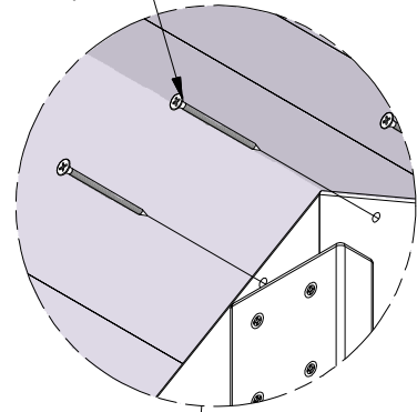
091 (x12) SCREW - 2 1/4"
