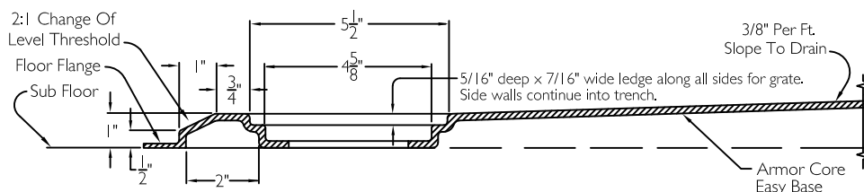
CROSS SECTION OF SHOWER BASE
