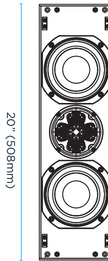
5.75" (146.05mm) Width OW53QT Front View
