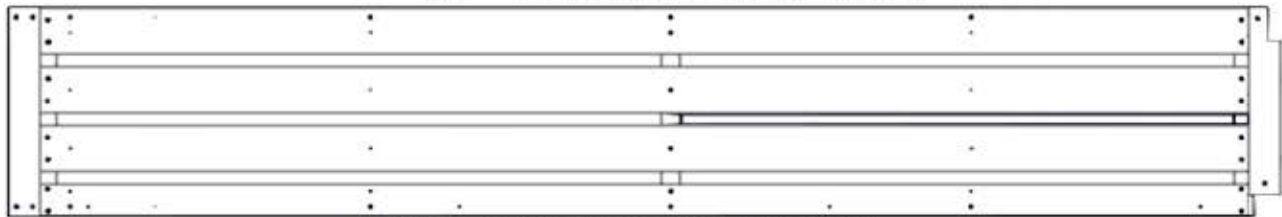
TB01 TABLE ASSEMBLY - W2A04325 (x1) 2 1/16"x14 7/8"x89 1/2" (52x378x2274)
