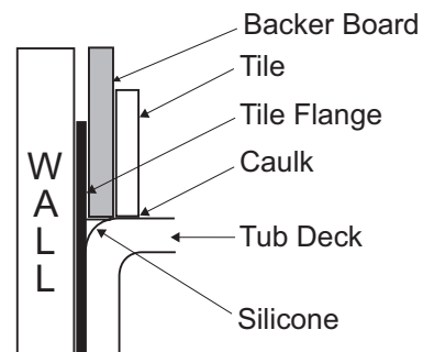
Tile Flange is also available as a field installation kit, sold separately, for onsite installation.
