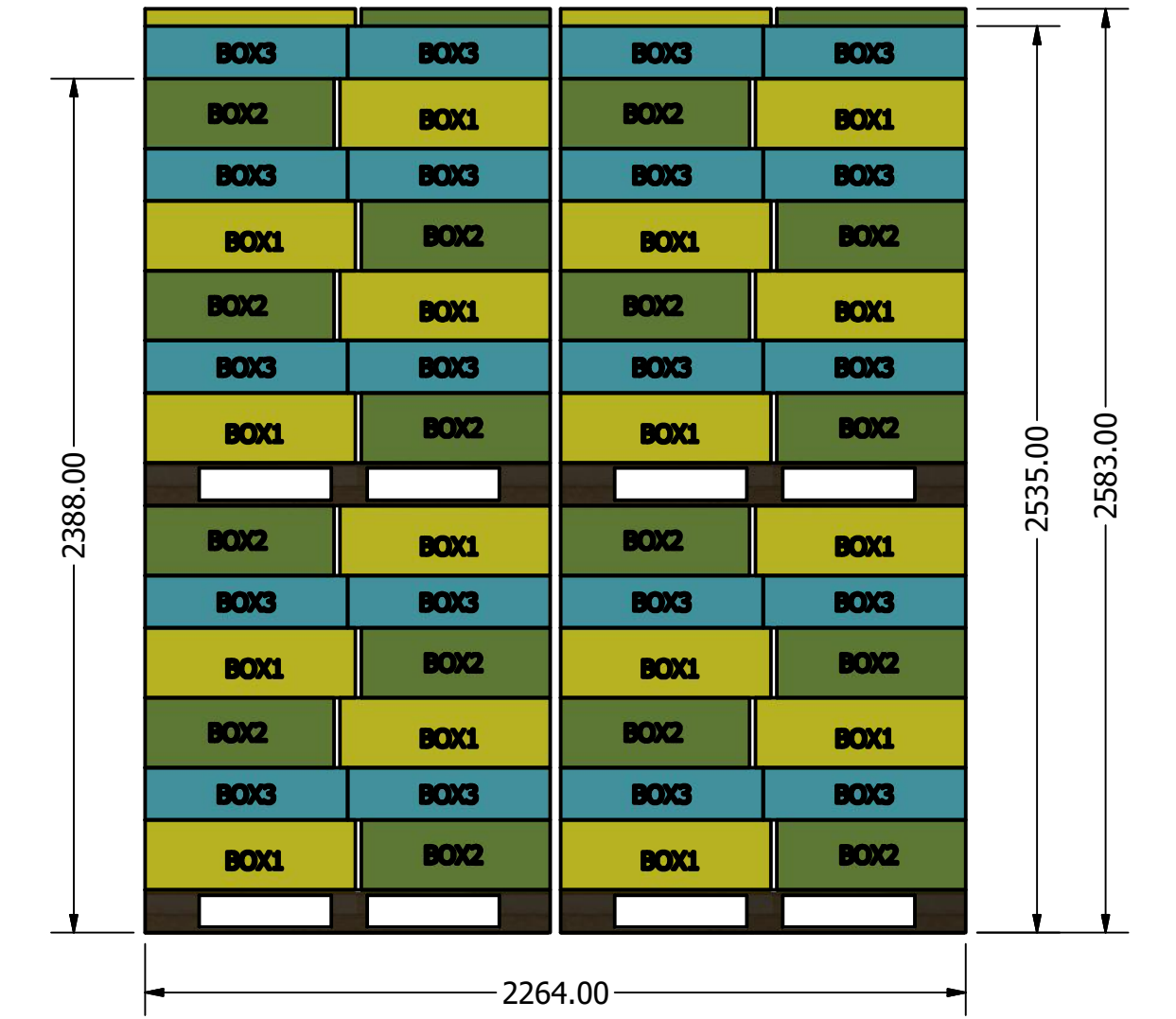
End view
