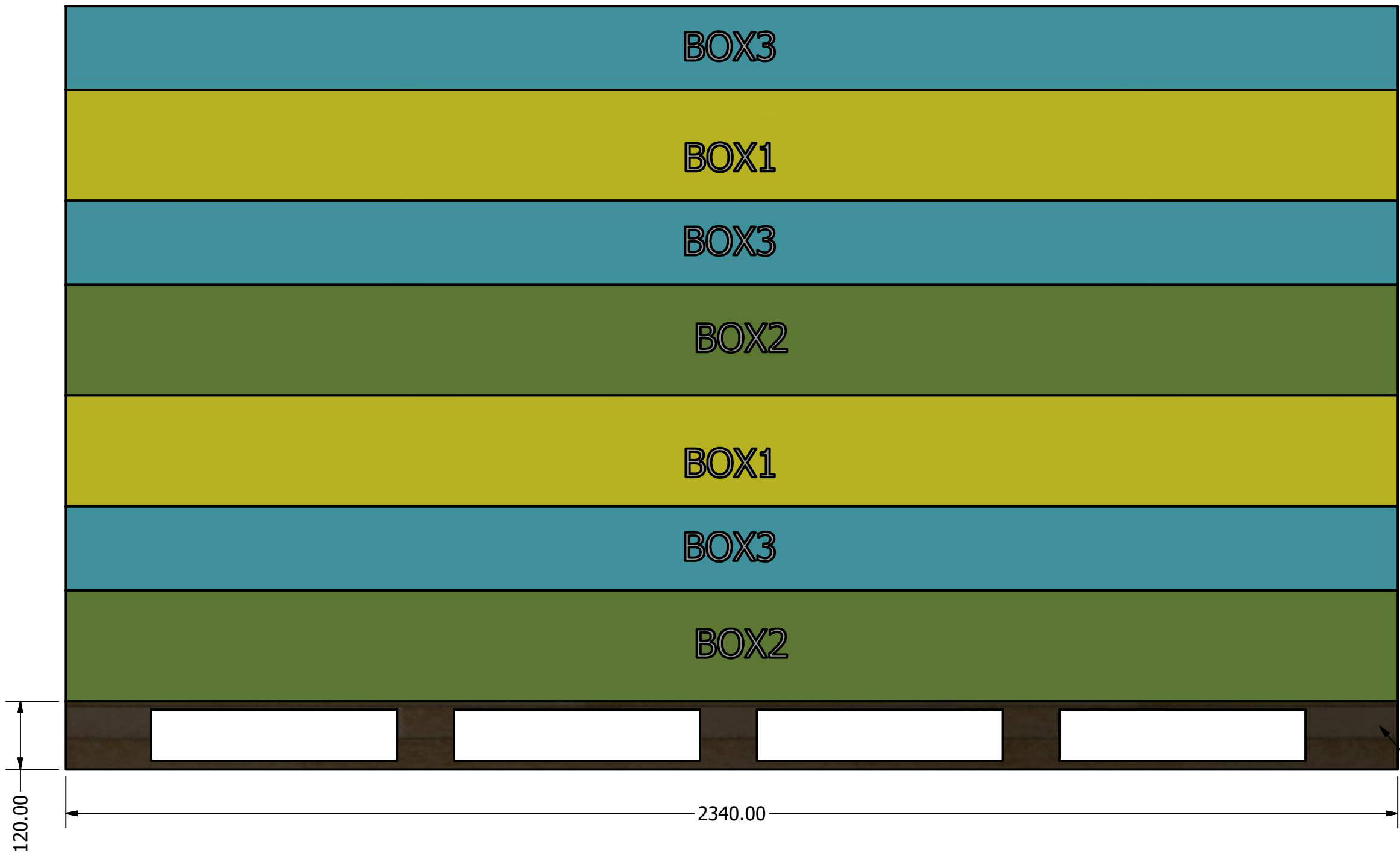
Side View
