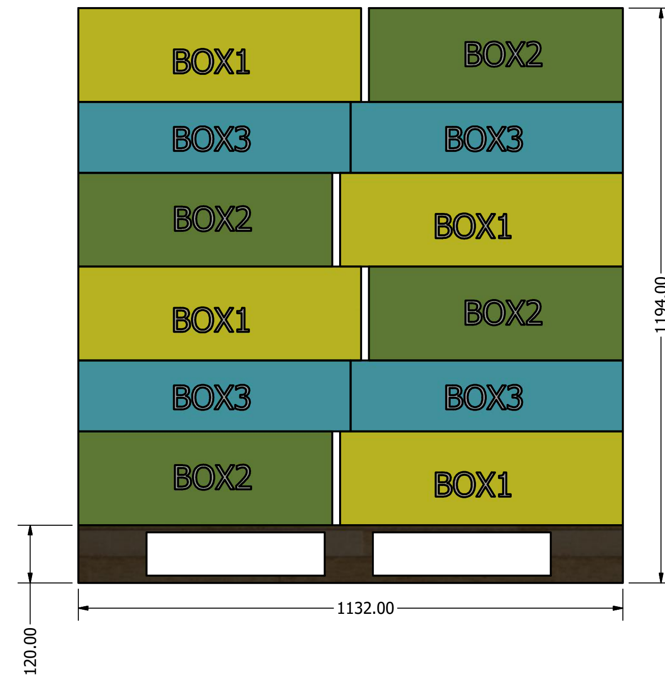
End View
