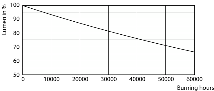
Lumen Maintenance Diagram - 40T8/COR/96-5CCT/MF55LS/G/FA8-R17D 10/1
