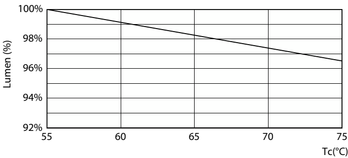
Lumen Maintenance Diagram - 40T8/COR/96-5CCT/MF55LS/G/FA8-R17D 10/1
