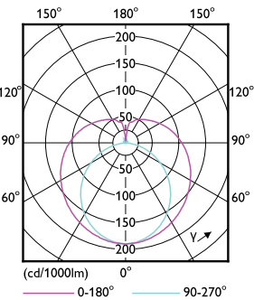
Light Distribution Diagram - 40T8/COR/96-5CCT/MF55LS/G/FA8-R17D 10/1
