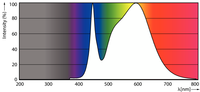
Spectral Power Distribution Colour - 40T8/COR/96-5CCT/MF55LS/G/FA8-R17D 10/1
