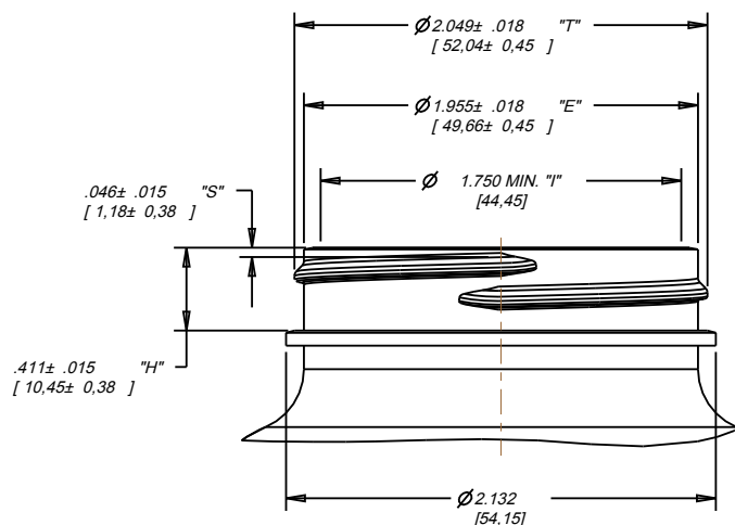
DETAIL A M53-400 NECK FINISH 6 T.P.I., 1 THREAD TURN .250 MIN "I" DEPTH SCALE 2.000
