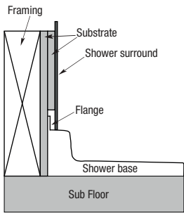
Flange Details: (U.S.)
