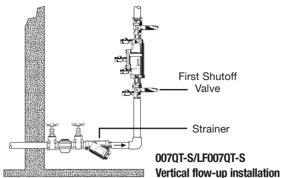
Vertical flow-up installation
