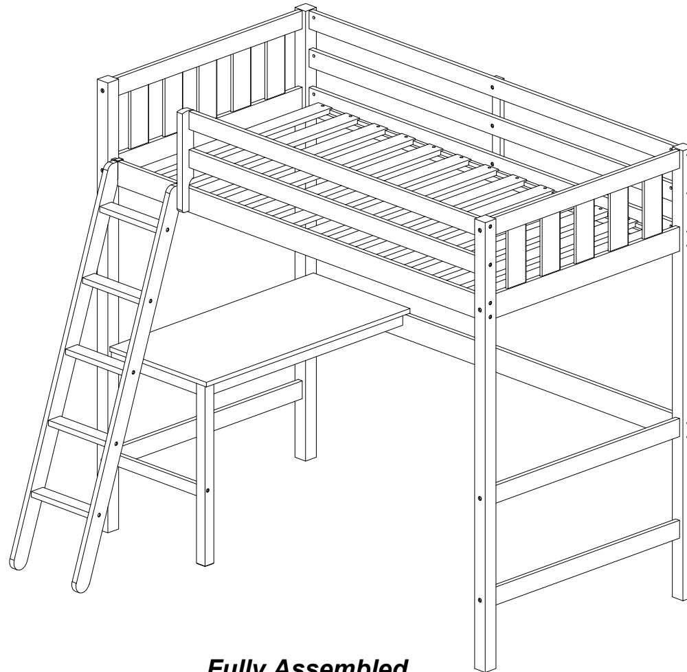
Fully Assembled LOFT BED WITH TABLE
