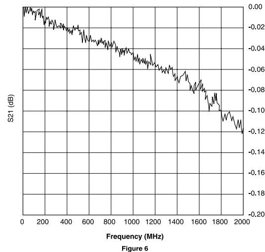
S21 vs Frequency for an APG gas tube surge arrestor
