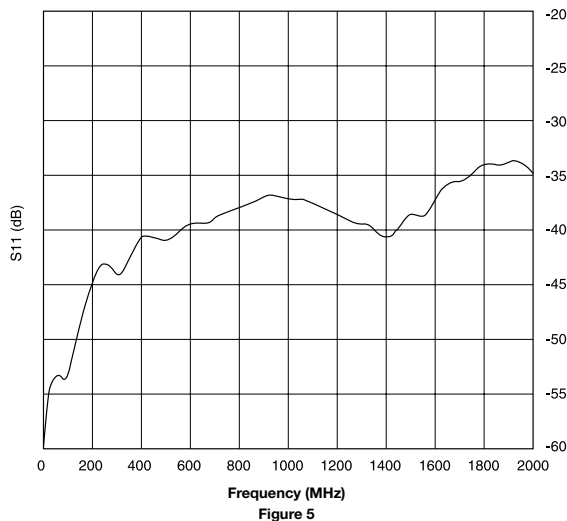
S11 vs Frequency for an APG gas tube surge arrestor
