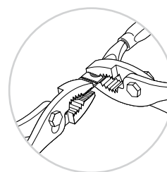
Snap off pre-scored lug for one hole option
