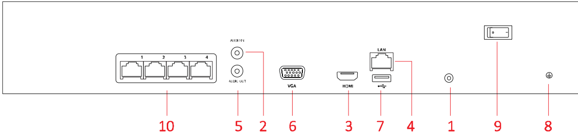
ERI-K108-P8 Rear Panel
