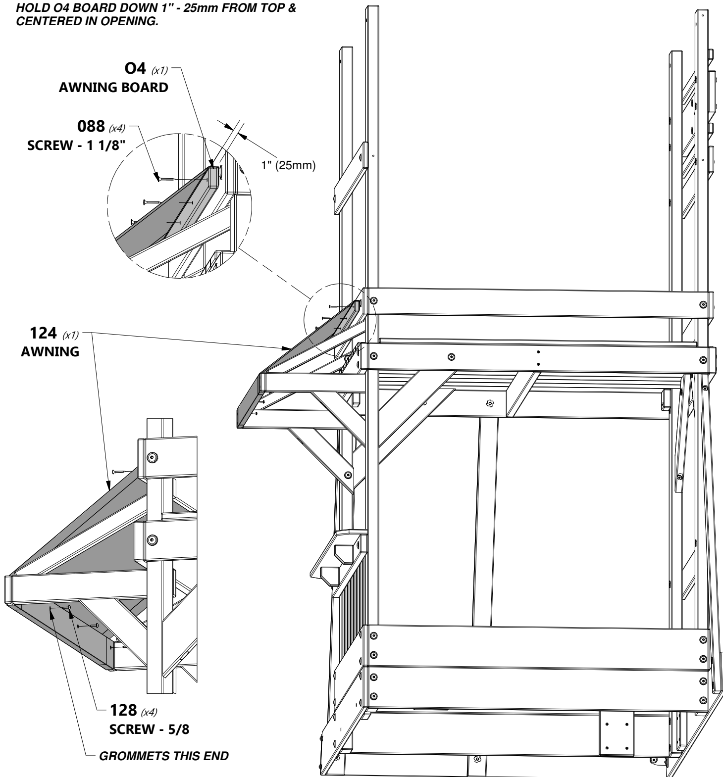
A6P00124 | AWNING (1)
