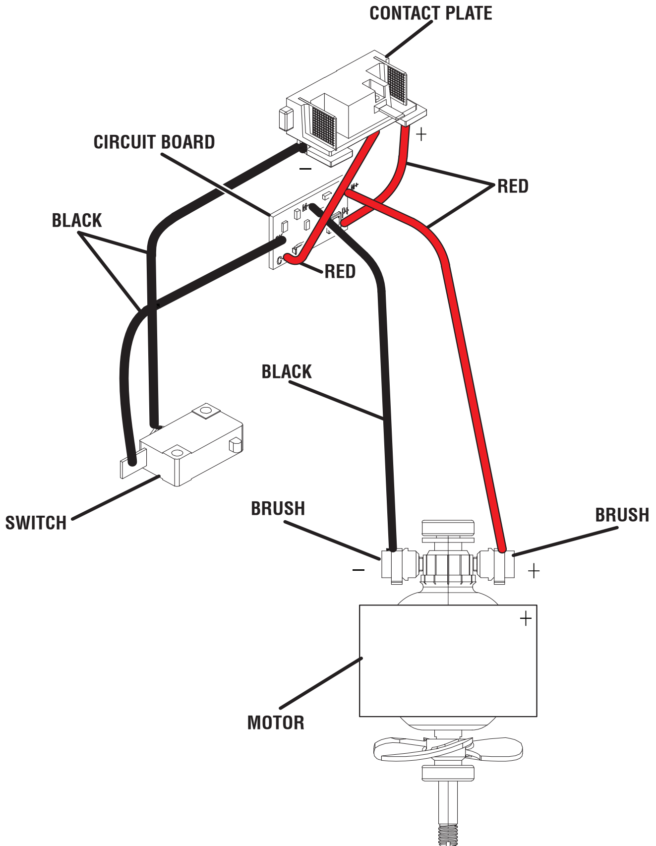
WIRING DIAGRAM
