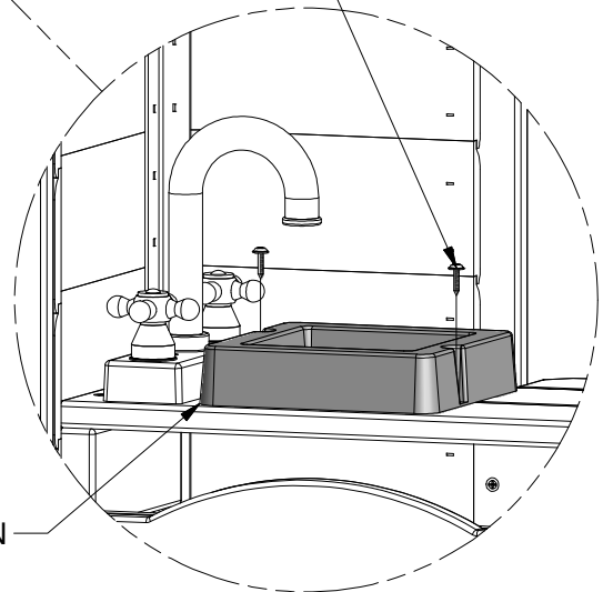
SURFACE MOUNT BASIN
