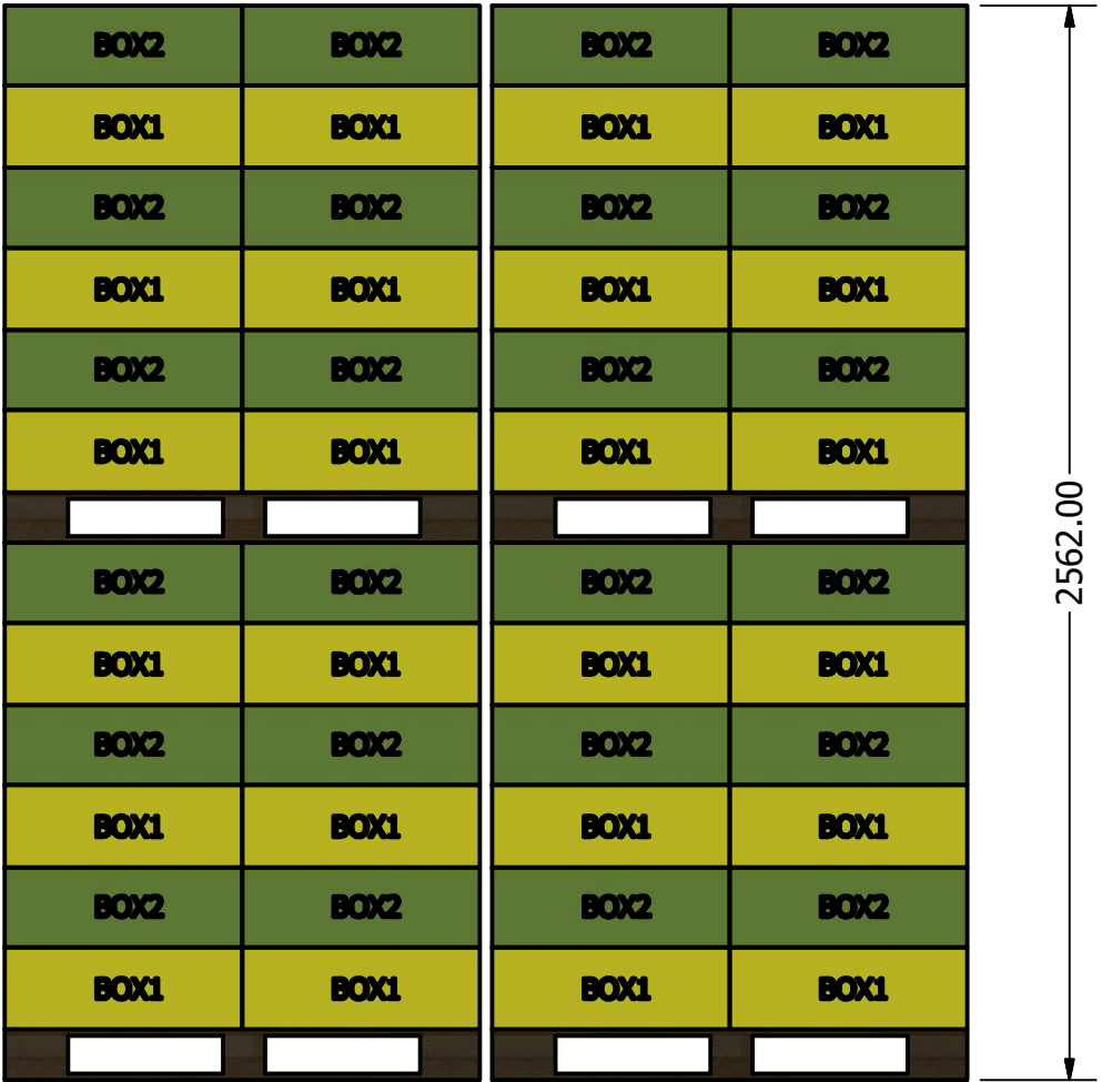
End view
