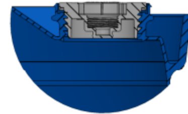
DETAIL C SCALE 1 : 2 2" BUTTRESS CLOSURE 5 T.P.I.
