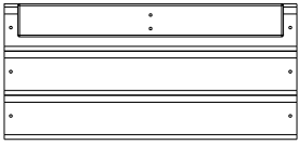
WP7 | UPPER REAR CENTER WALL - W2A02989 (x1) | 1 1/2"x21 1/8"x9 3/4" (38x536x248)
