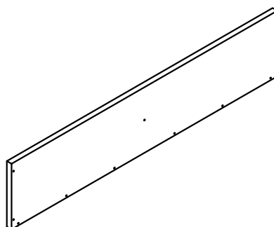
BOTTOM BACK PANEL QTY 1
