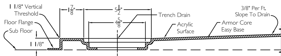
CROSS SECTION OF SHOWER BASE
