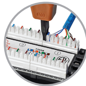
PUNCH DOWN
