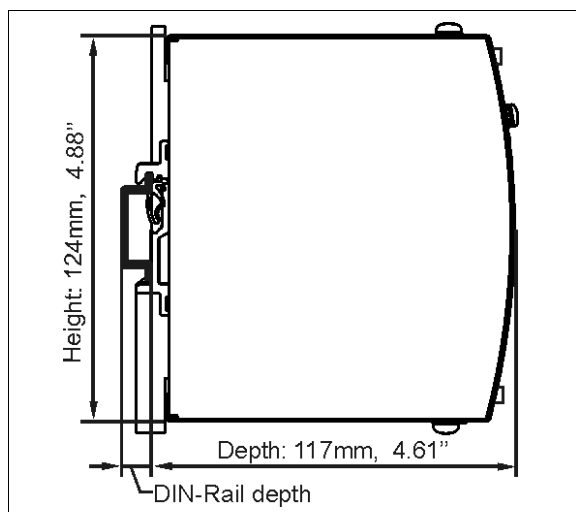
Fig. 20-2 Side view
