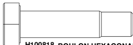
H100818 BOULON HEXAGONAL M12 x 50 mm WZ (x6) M12x 50mm
