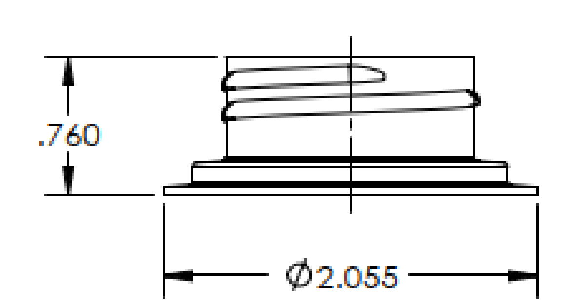
Ⓕ 38mm SP-400 SCREW FINISH "M" STYLE THREAD WITH 1-1/2 TURNS
