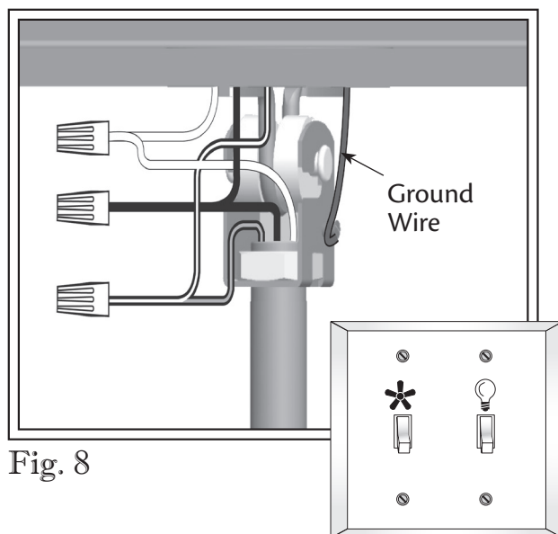
Wire Connector
