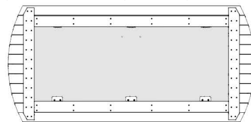
WP04 ASSEMBLAGE DE PANNEAU MURAL - W2A04794 (x1) 2 3/8"x35 5/8"x74 9/16" (60x906x201)
