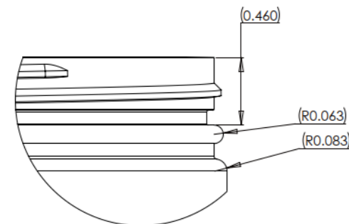
DETAIL C SCALE 2.5 : 1
