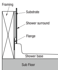
Flange Details: (U.S.)
