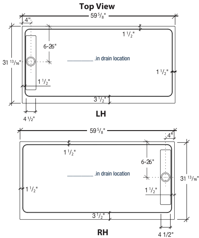
Drain Details: (U.S.)
