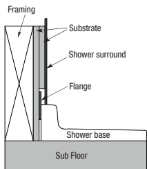
Flange Details: Fire Rated Walls (U.S.)
