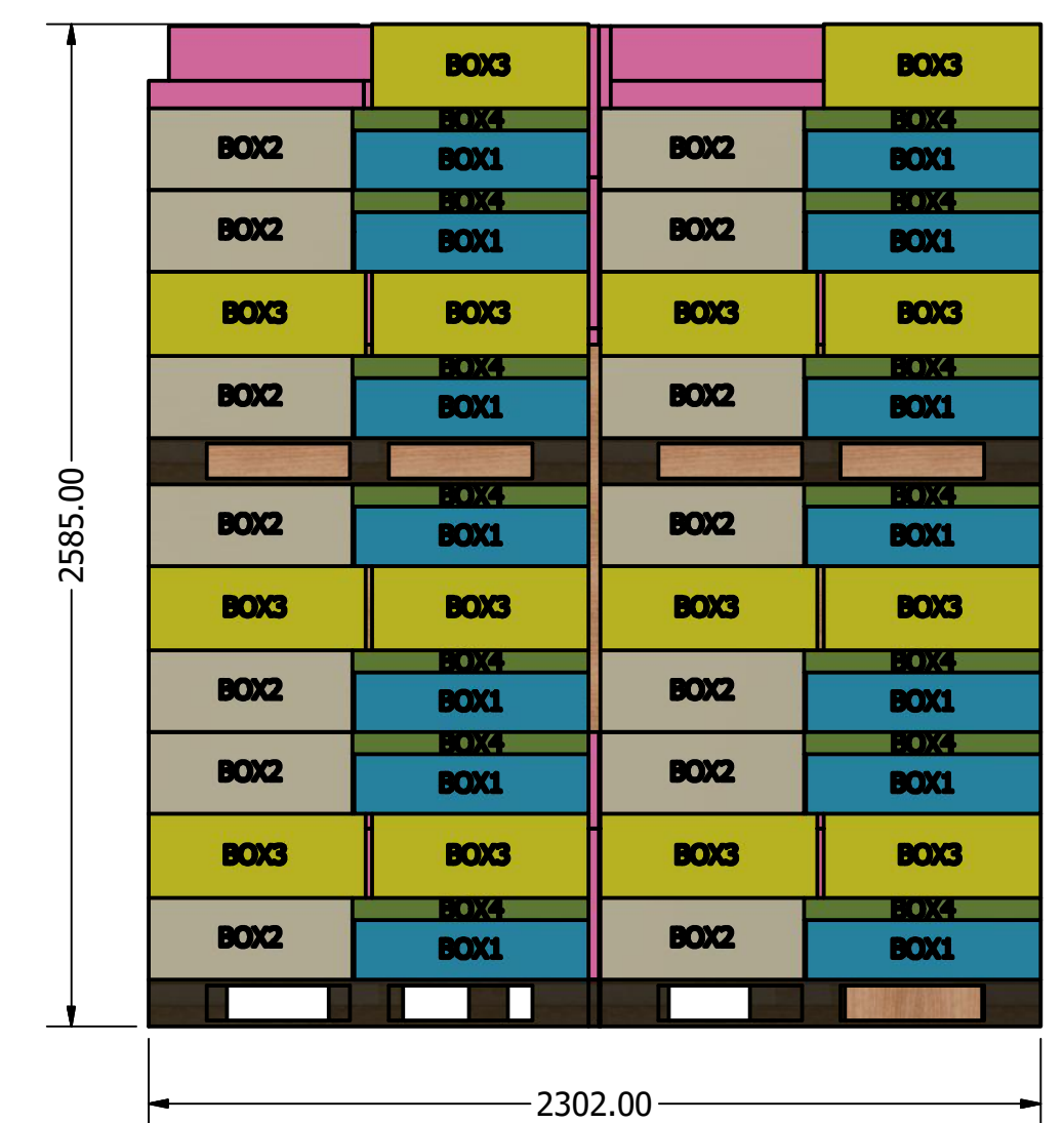
End view
