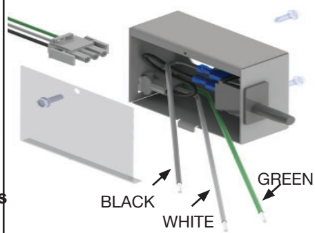
FIGURE 31 - ELECTRICAL CONNECTIONS / MOLEX CONNECTOR
