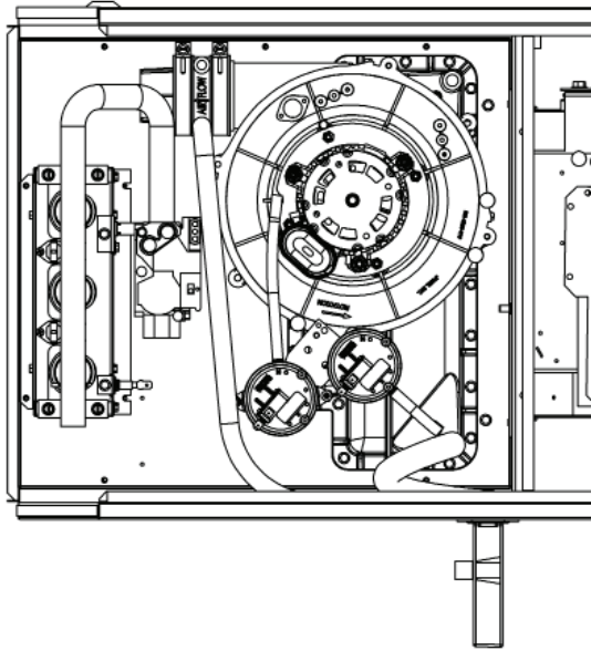
FIGURE 17 - HORIZONTAL LEFT VENT AND DRAINING OPTION
