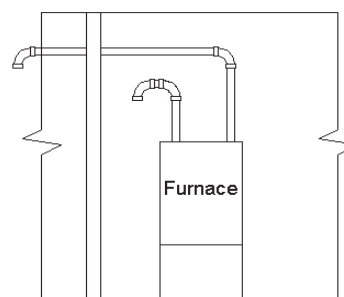
FIGURE 7 - NON-DIRECT COMBUSTION AIR INLET
