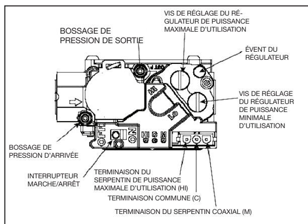
FIGURE 28 - SOUPE DE GAZ WHITE RODGERS 36G54
