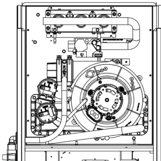
LEFT VENT - LEFT DRAIN INSTALLATION (EXTERNAL)
