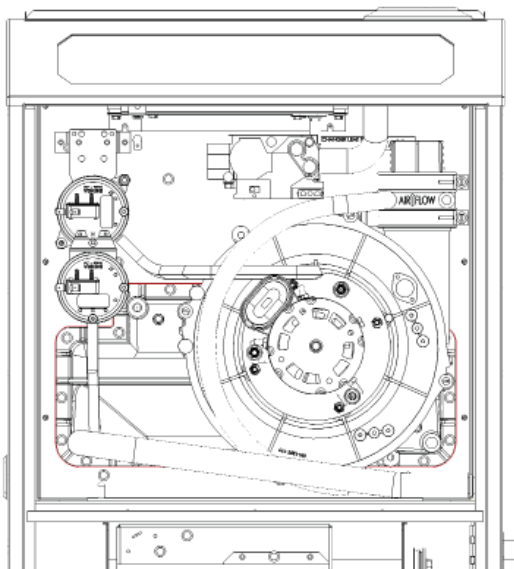
TOP VENT - RIGHT DRAIN INSTALLATION (INTERNAL)
