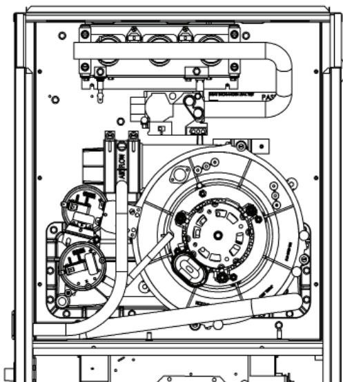
LEFT VENT - LEFT DRAIN INSTALLATION (INTERNAL)
