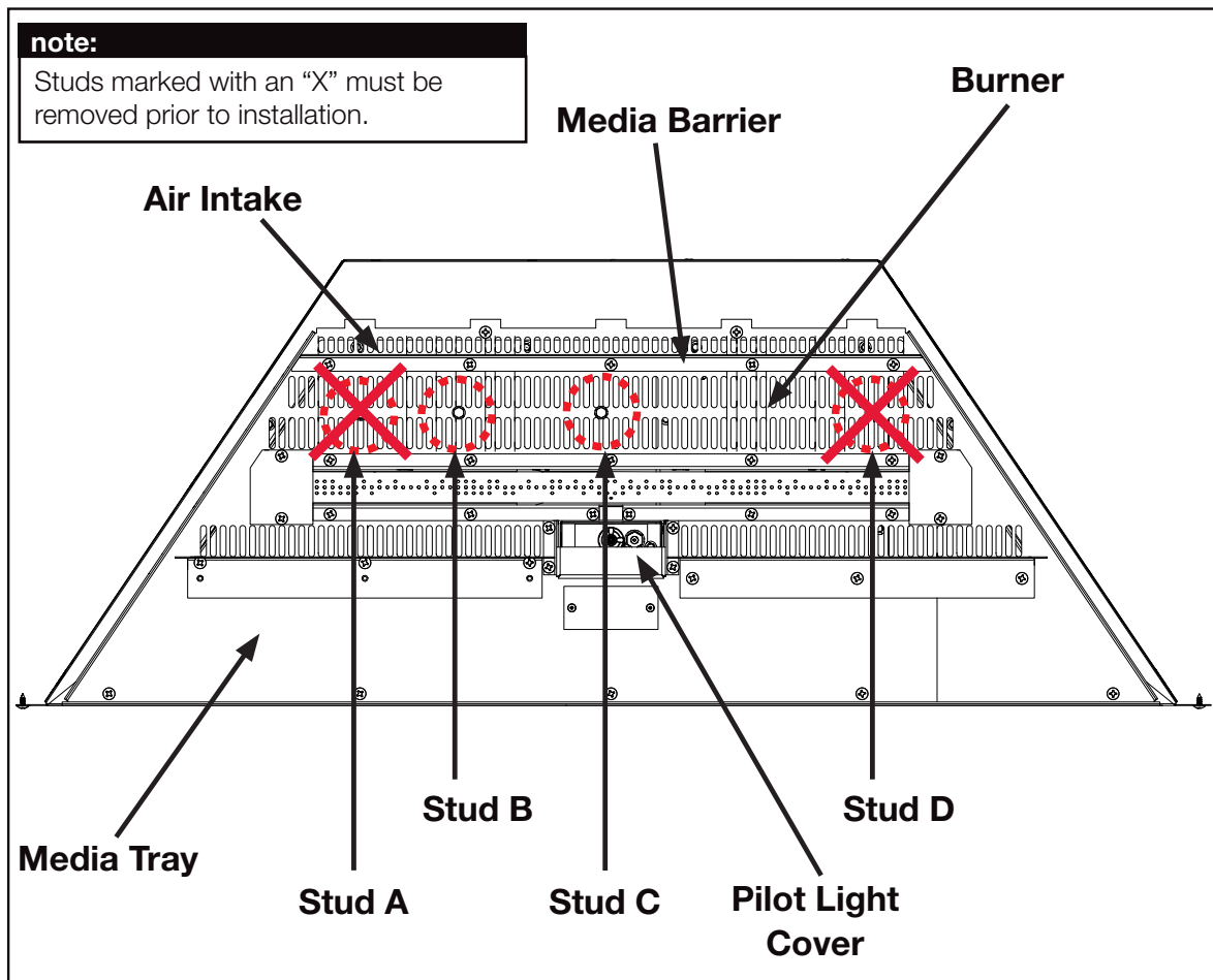
Burner Overview
