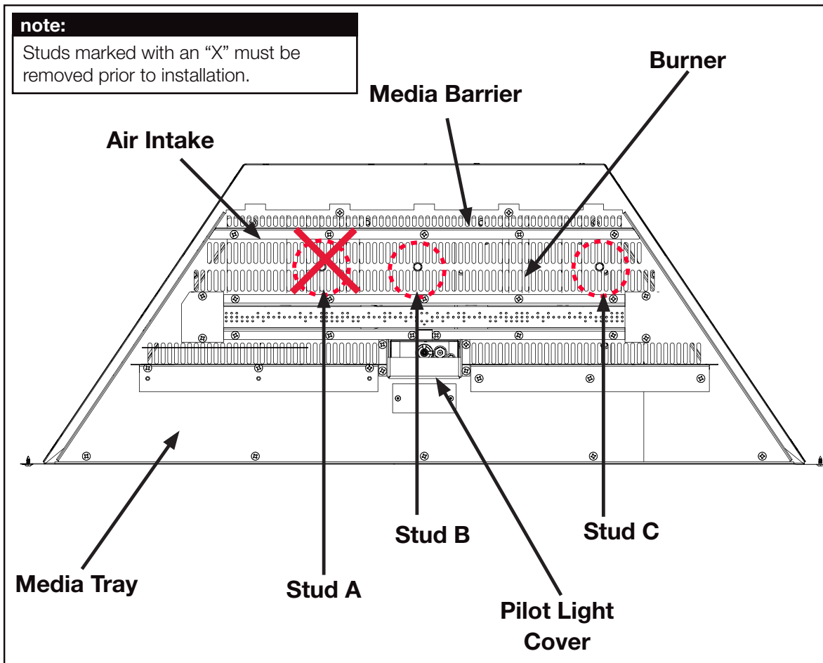
Burner Overview
