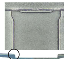
3M™ Polycarbonate Carrier 3000 R Series, either in 8 mm, 12 mm, 16 mm or 24 mm wide indicate sharper pocket opening.
