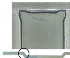
3M™ Polycarbonate Carrier 3000 R Series, either in 8 mm, 12 mm, 16 mm or 24 mm wide indicate sharper pocket opening.
