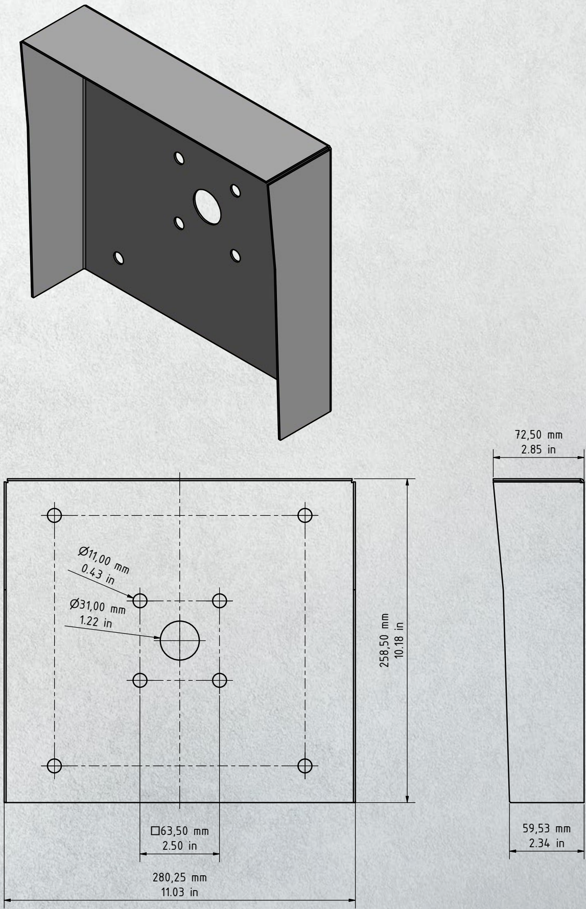
Protective hood for D21xKH
