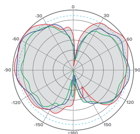
Elevation Radiation Pattern (Typical)
