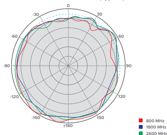
Azimuth Radiation Pattern (Typical)
