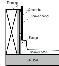
Flange Details: (U.S.)
