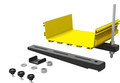
FiberGuide® New Threaded Rod Bracket Kit, 5/8in for 4x12in System
