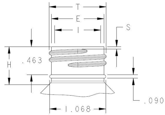
DETAIL A SCALE 3/2
