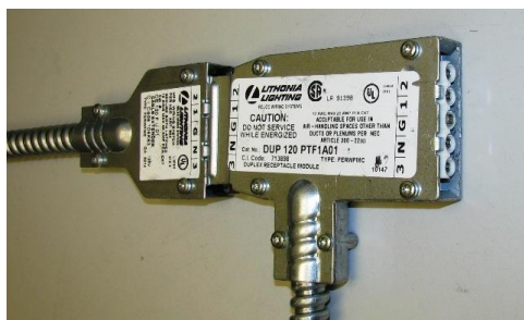
SYSTEM 820 without cap on unused opening.
