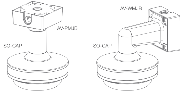
Ceiling Mount Configuration
