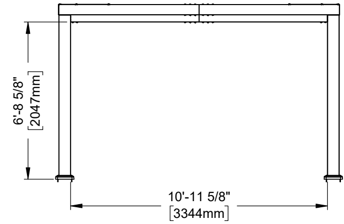
14' X 12' MODERN METAL PERGOLA FOOTPRINT
