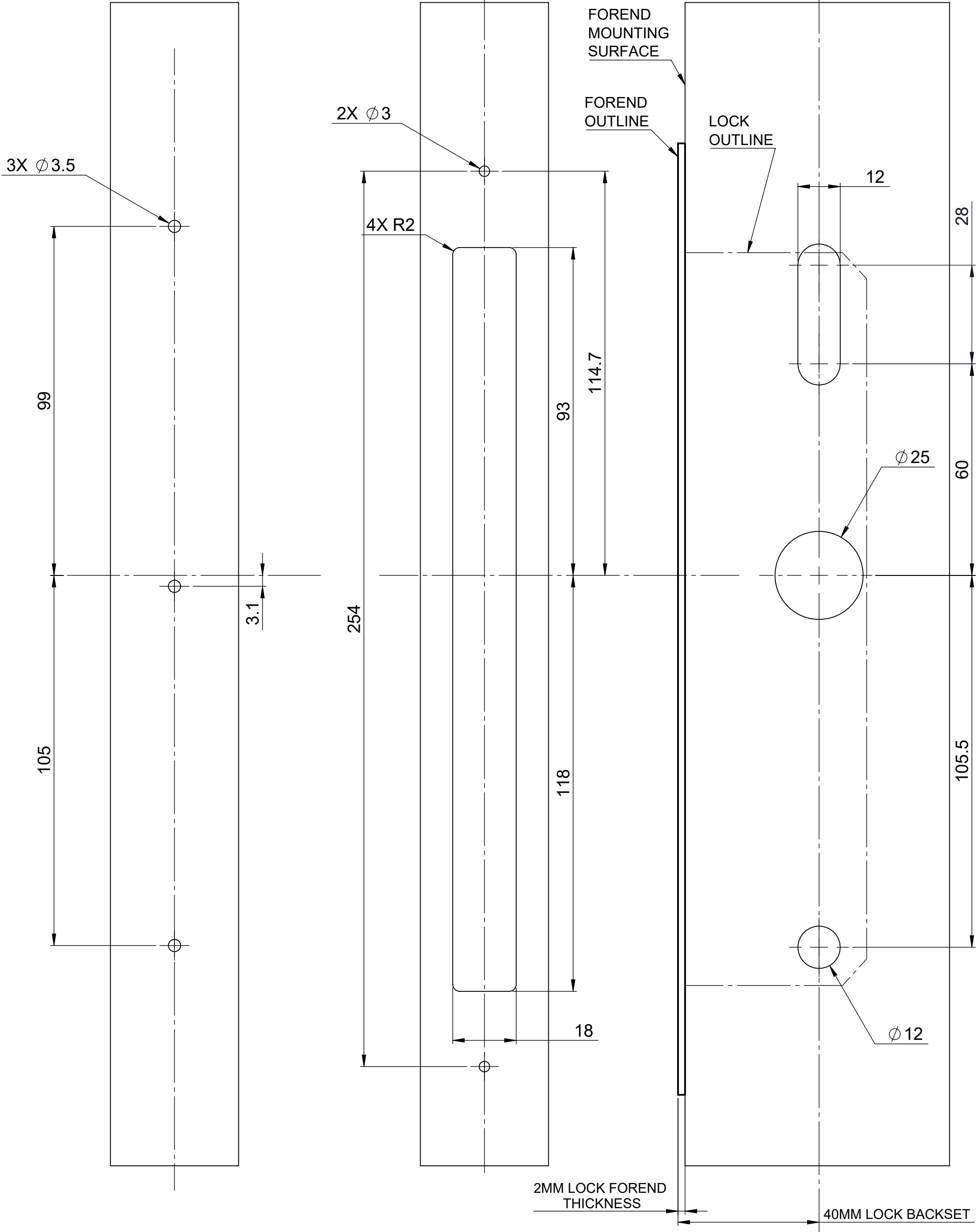
FRONT VIEW
