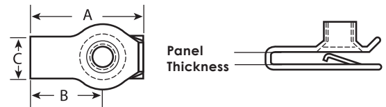
Multi-Thread "U" Nut
